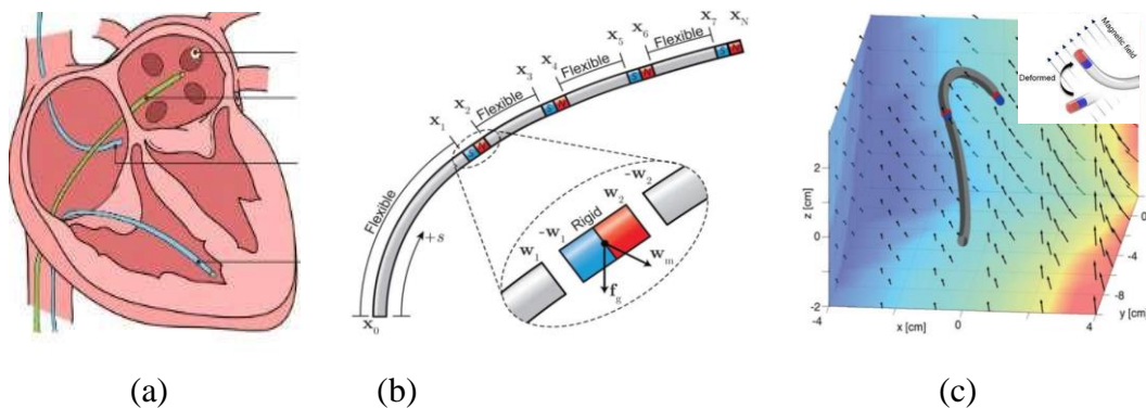
Figure 1: Magnetically guided soft catheters : (a) Catheter motion guidance for treatment of atrial fibrillation in the heart; (b) Magnetic catheter comprising four flexible, non-magnetic and four rigid, permanent-magnetic segments and (c) Principle of magnetic control using the forces and torques generated by the interactions between embedded permanent magnets and the magnetic vector field.
